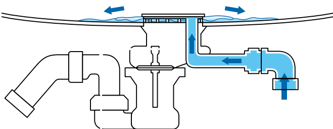
The inlet comes with a backflow preventer and pipe interrupter.
