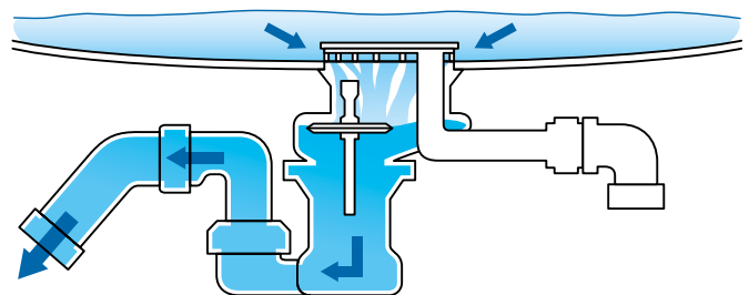
By opening the valve cone (can be electronically controlled if desired) the service water flows off as usual.
